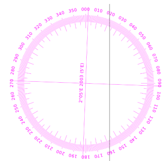
Figure 2: Magnetic variation.
